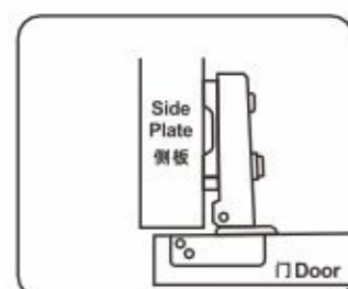
HB06A Full cover 全盖
