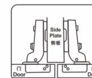
HBH1193 Half cover 半盖
