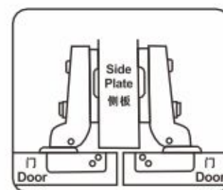
HBS183B Half cover 半盖
