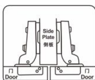
HBE35B Half cover 半盖
