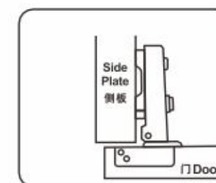
HB126A Full cover 全盖
