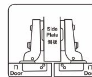
HB127B Half cover 半盖
