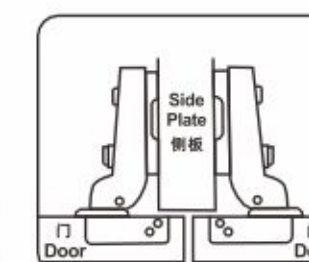
HB116B Half cover 半盖
