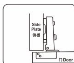
HBE35A Full cover 全盖
