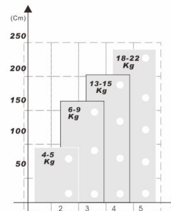
每扇门所需铰链数量 (板材厚19-24MM) Number of cup hinges per door (with 18MM chipboard)
