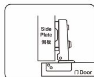
HB109A Full cover 全盖
