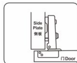
HBS131A Full cover 全盖
