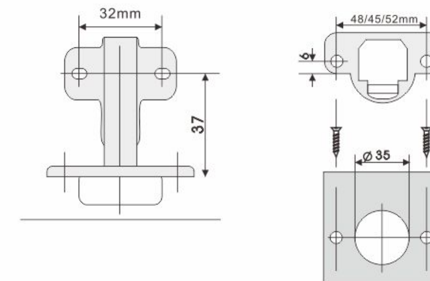
配自攻螺丝 with self-tapping screw 配欧洲螺丝 With euro screw 配双桥胶套螺丝(5mm) With dowel(5mm) 配M8胶粒螺丝(8mm) With dowel(8mm) 配M10胶粒螺丝(10mm) With dowel(10mm)
