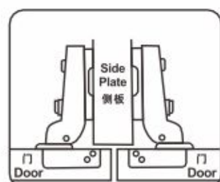
HB06B Half cover 半盖
