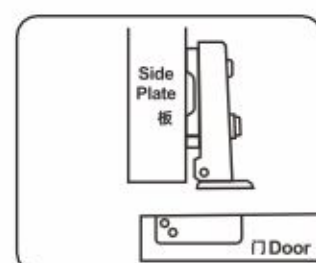
Full cover 全盖
