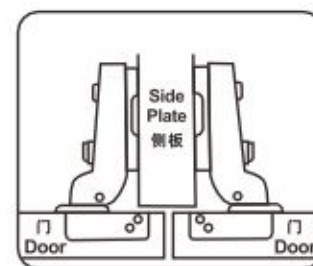
HBE31B Half cover 半盖
